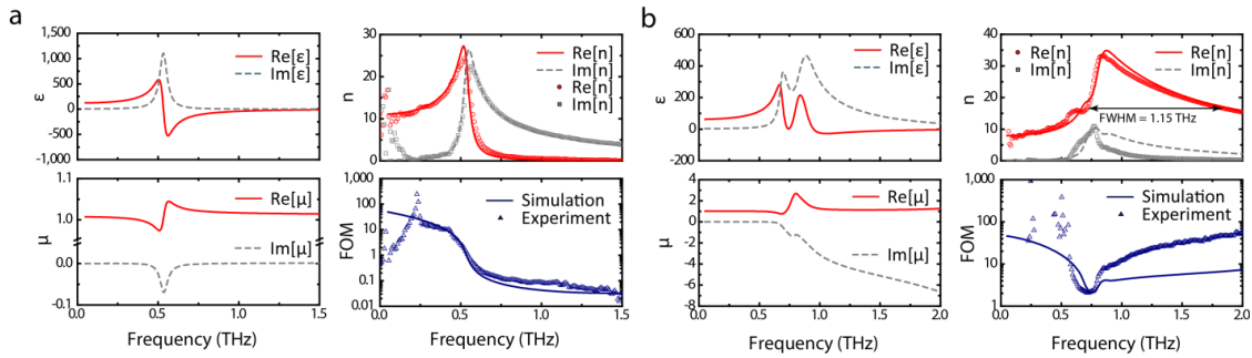
Figure 2: (a) Effective permittivity (top left), permeability (bottom left), refractive index (top right), and figure of merit (bottom right) for a single-layer metamaterial (b) Effective parameters for a five layer metamaterial
